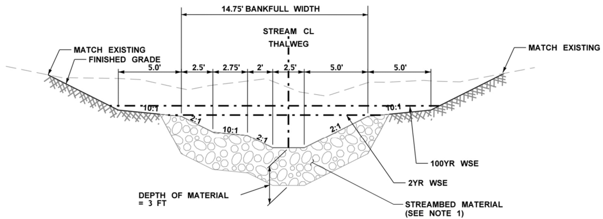
TYPICAL POOL RT SECTION (E) NTS
