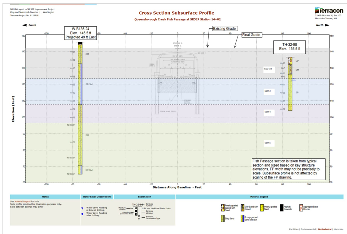
Figure 7-1: Subsurface cross-section of the proposed Queensborough Creek fish passage at SR 527
